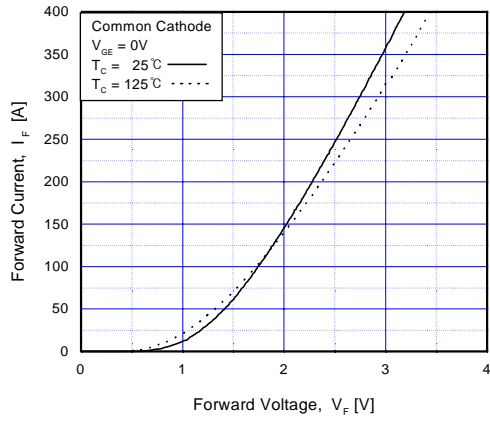
Fig 19. Forward Characteristics
